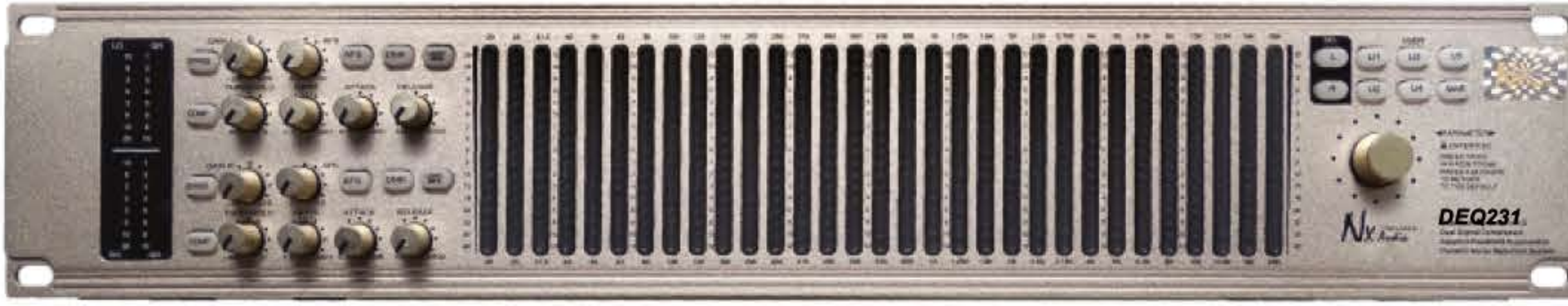
DEQ231 Stereo Digital Graphic Equalizer with Compressor & Feedback Suppression
